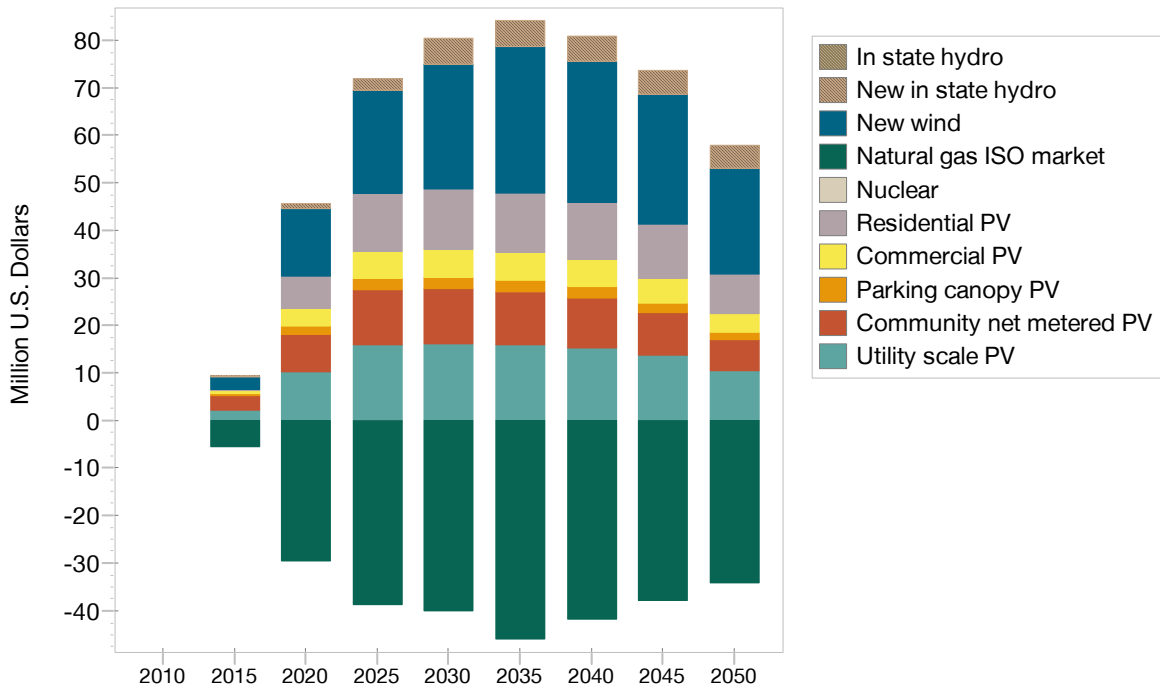
Figure 21. Annual discounted costs for electricity generation in the SDP scenario, compared to the Reference scenario.
